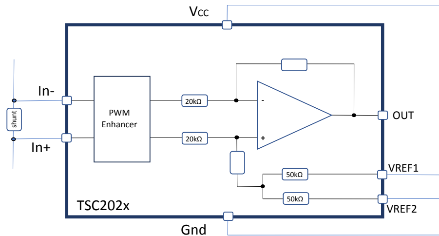
Figure 56. Split supply
