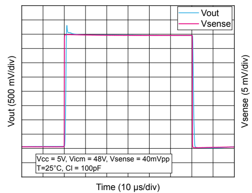
Figure 36. Large signal response with V_{CC} = 5V (TSC2022)
