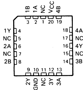
SN54HC00 . . . FK PACKAGE
