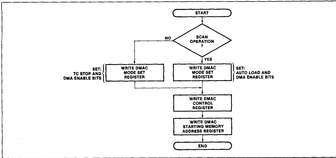
Figure 24. User DMA Channel Initialization Flowchart
