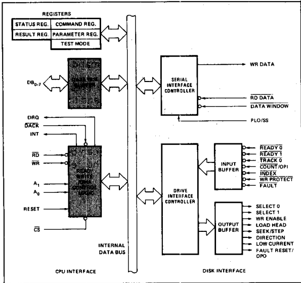
Figure 3. 8271 Block Diagram Showing CPU Interface Functions
