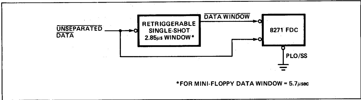
Figure 6. Single-Shot Data Separator Block Diagram
