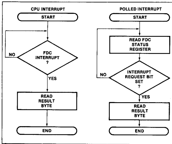
Figure 18. Getting the Result
