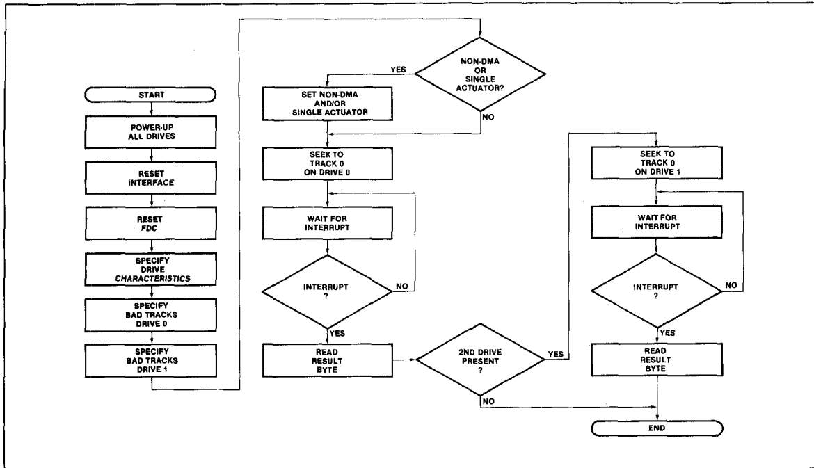
Figure 19. Initialization of the 8271 by the User
