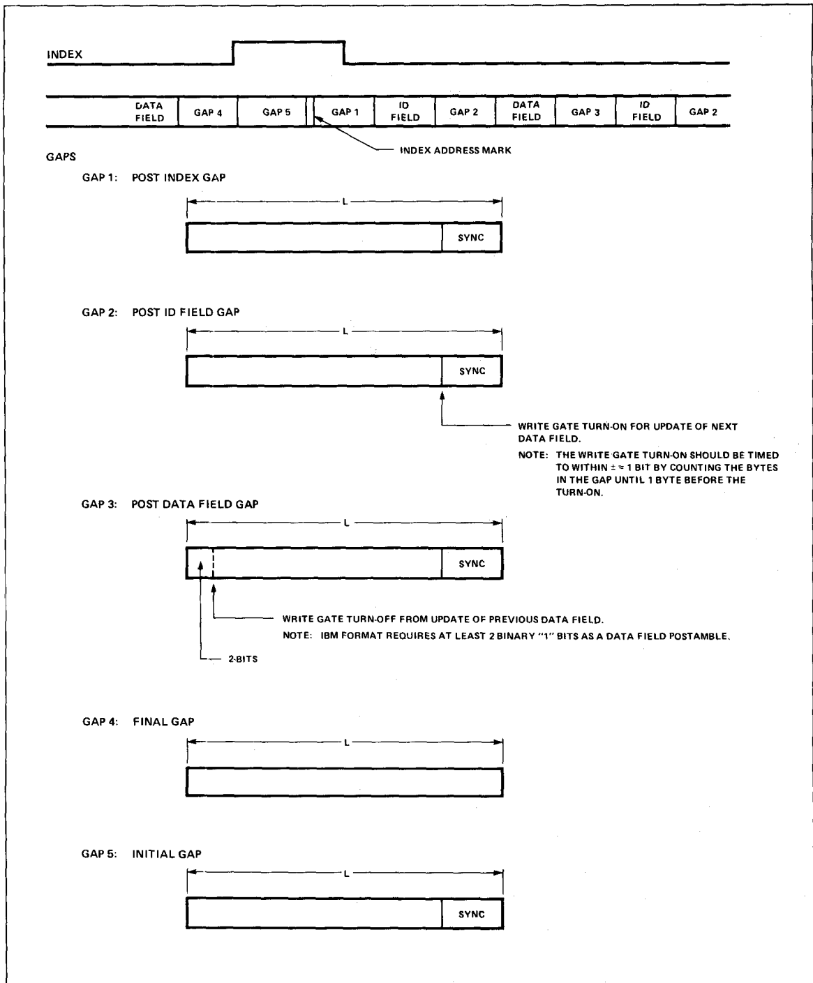
Figure 21. Track Format
