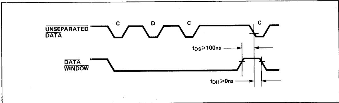
Figure 7. Single-Shot Data Window Timing
