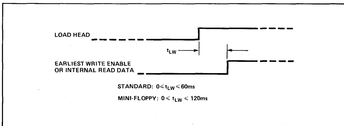
Figure 14. Head Load to Read/Write Timing
