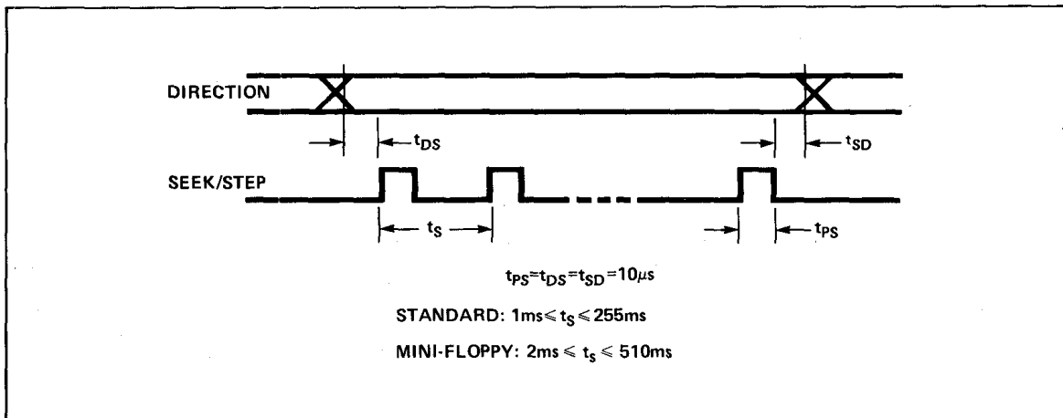
Figure 11. Seek Timing
