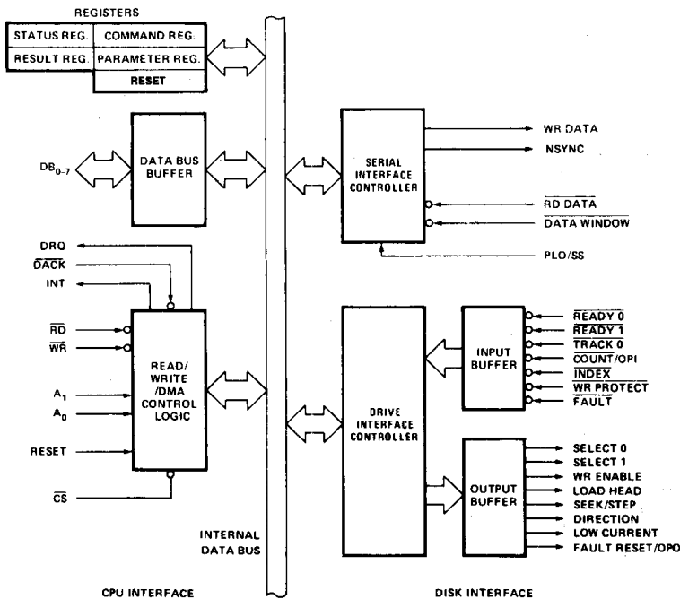
Figure 1. Block Diagram
