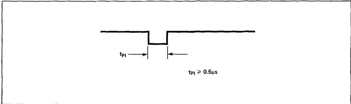
Figure 15. Index Timing
