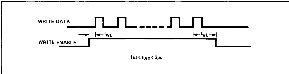
Figure 10. Write Enable Timing
