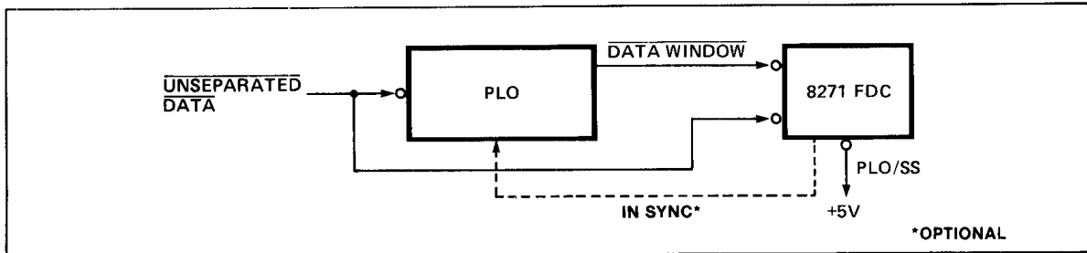
Figure 8. PLO Data Separator Block Diagram
