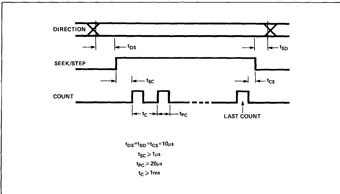
Figure 12. Seek/Step/Count Timing
