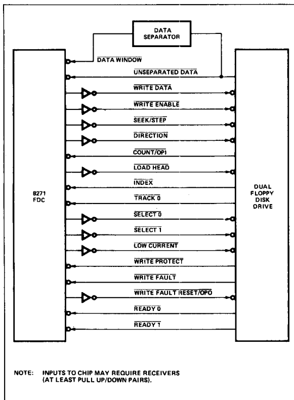
Figure 5. 8271 Disk Drive Interface
