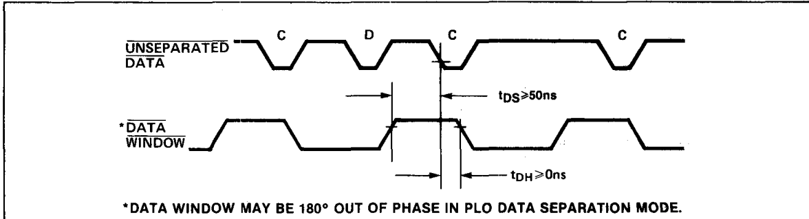
Figure 9. PLO Data Window Timing
