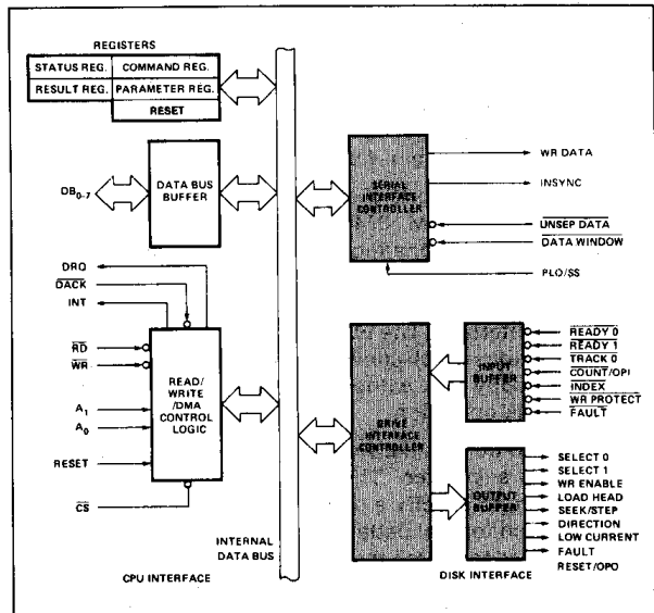
Figure 4. 8271 Block Diagram Showing Disk Interface Functions
