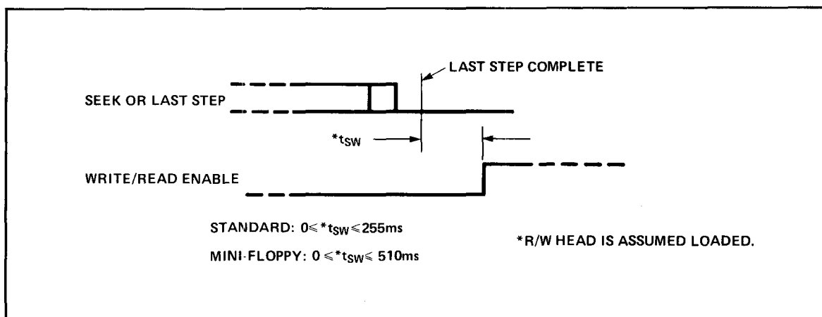
Figure 13. Head Load Settling Timing
