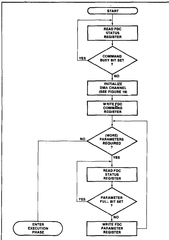
Figure 16. Passing the Command and Parameters to the 8271
