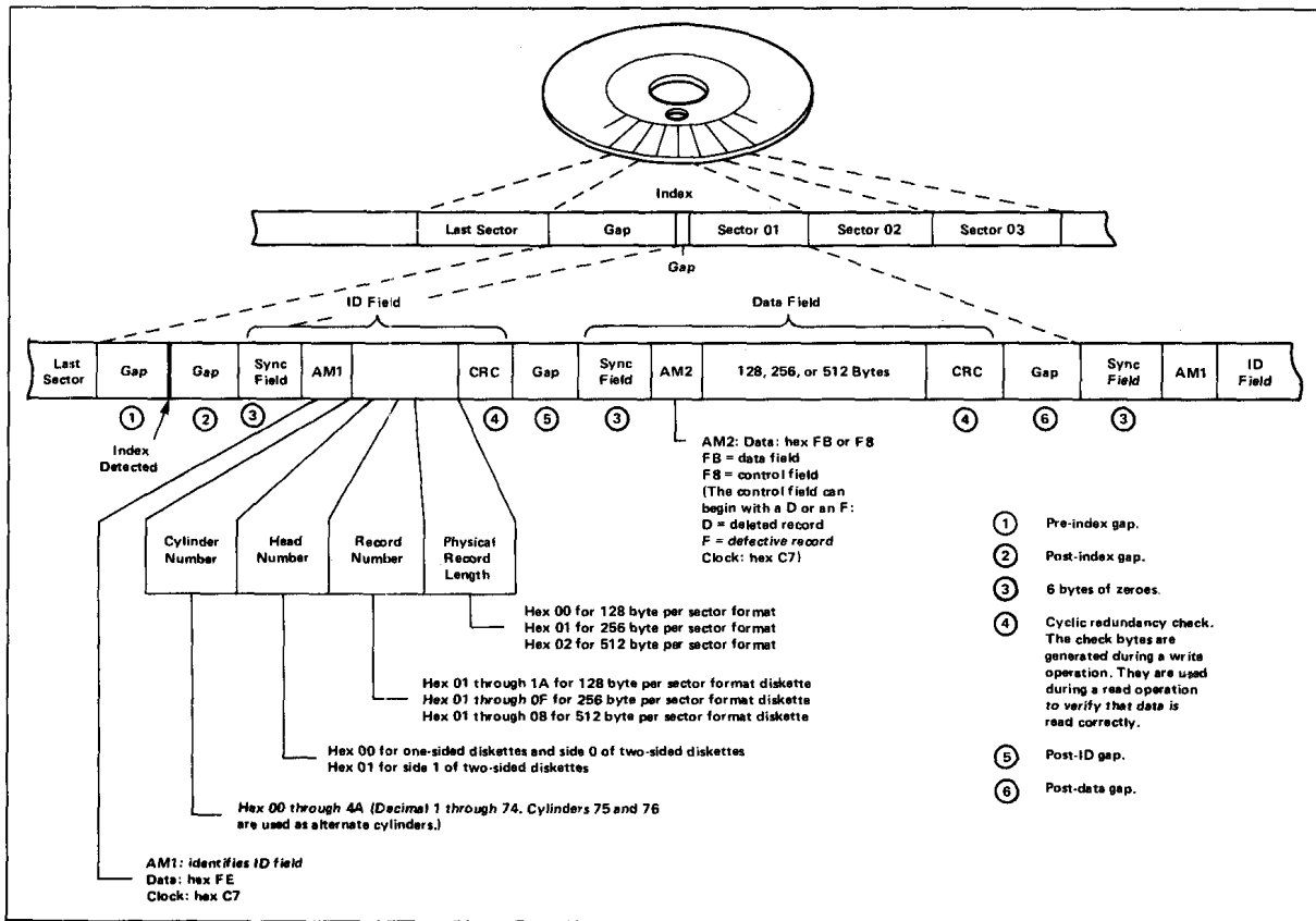
Figure 20. Track Format
